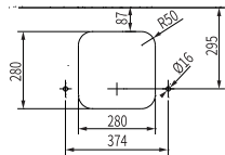
台面切割孔/ Holes cutting drawing
