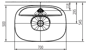
台面切割孔/ Holes cutting drawing
