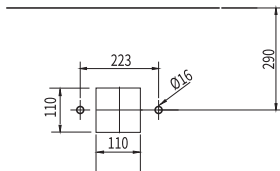
台面切割孔 Cutting hole of floor
