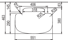
台面切割孔 Cutting hole of floor
