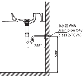
切割孔图纸 / Holes cutting drawing
