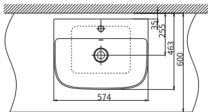
切割孔图纸 / Holes cutting drawing
