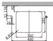
切割孔图纸 / Holes cutting drawing
